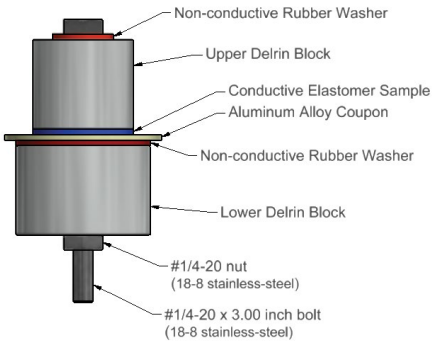
Figure 2-1: Test Fixture
