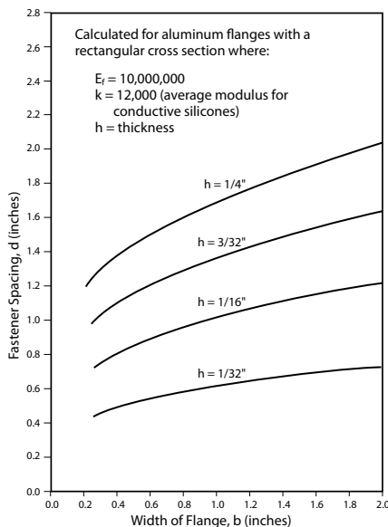
Figure 1-13. Fastener Spacing
