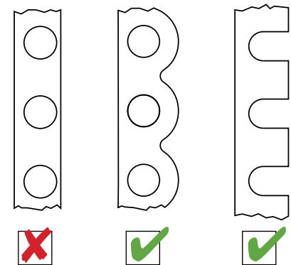
Figure 1-5. Ears or Slots in Sheet Metal Flanges or Flat Gaskets
