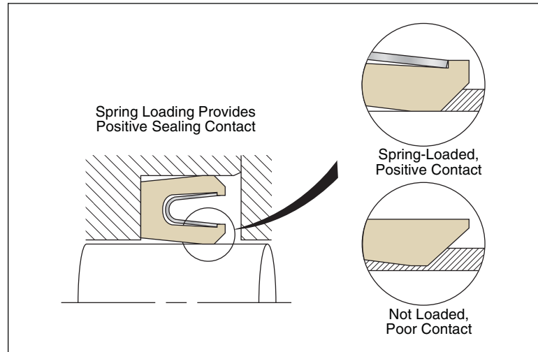
Figure 2-13. Spring Loading
