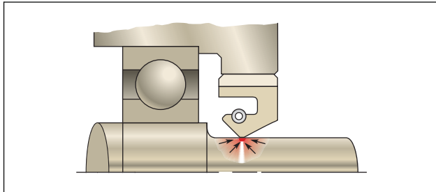
Figure 2-9. Internal Pressure
